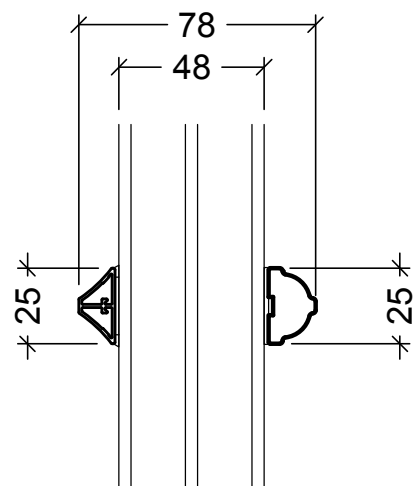
Ⓝ 3014.1109 without glazing bars
