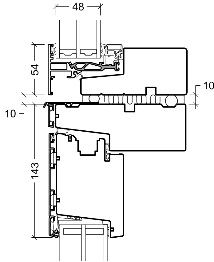
VELFAC 200 Energy / Ribo alu Outward opening
