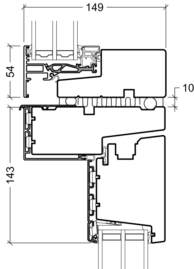
VELFAC 200 Energy / Ribo alu Inward opening
